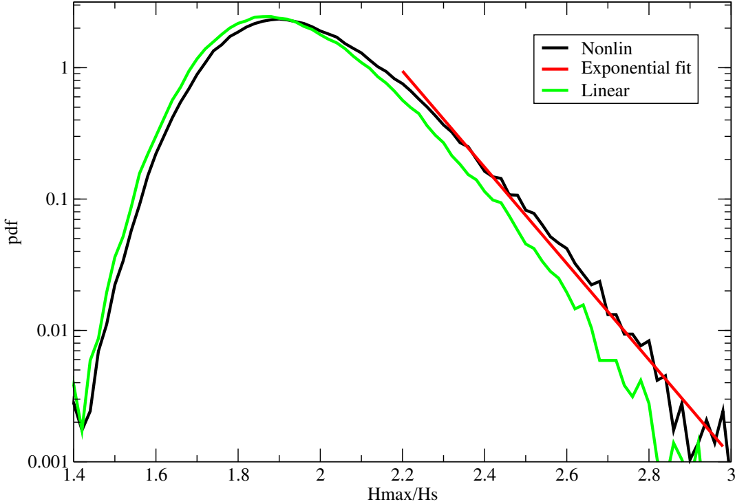
Figure 8.8 Global maximum wave height distribution obtained by a random draw of H_{max} for given number of waves and given skewness and kurtosis. Including skewness and kurtosis shows that the tail of the distribution is exponential. The distribution according linear theory is shown as well.
