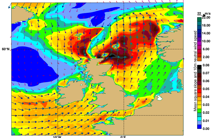
Figure 10.12 Mean Square Slope (colour shading), 10m Wind (arrows) on 23 March 2016, 6 UTC.
