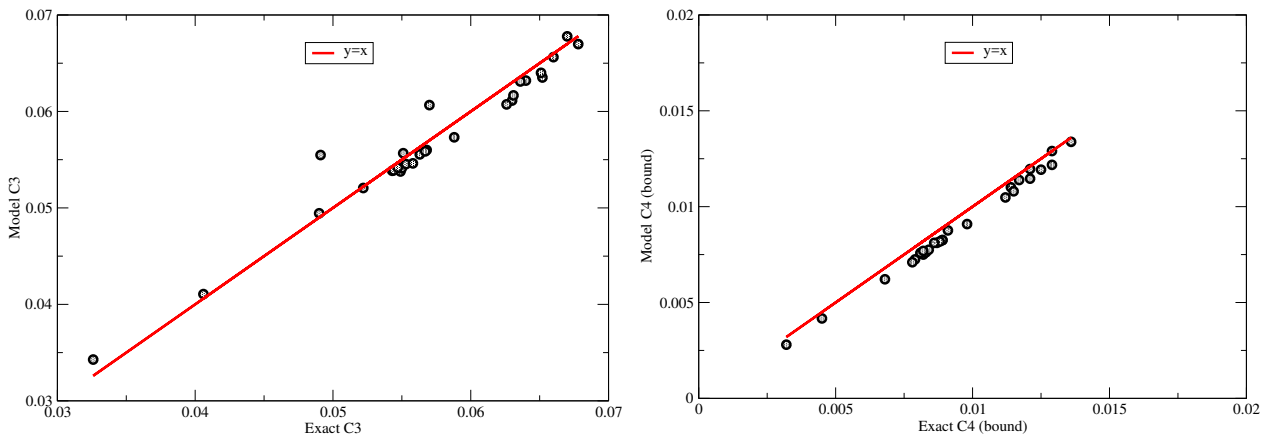
Figure 8.3 The left panel shows the comparison of parametrized skewness factor C_3^{bound} against exact computation from the Draupner and Andrea events, while the right panel shows the comparison for the kurtosis factor C_4^{bound} .
