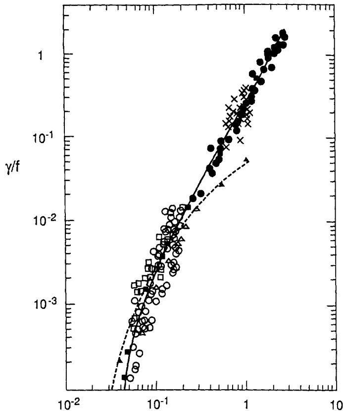
Figure 3.1 Comparison of theoretical growth rates with observations compiled by Plant (1982). Full line: Miles' theory; full squares: parametrization of Miles' theory (3.3); dashed line: the fit by Snyder et al. (1981). ( \beta_m = 1.2 , z_\alpha = 0.011 and \alpha = 0.0144 )
