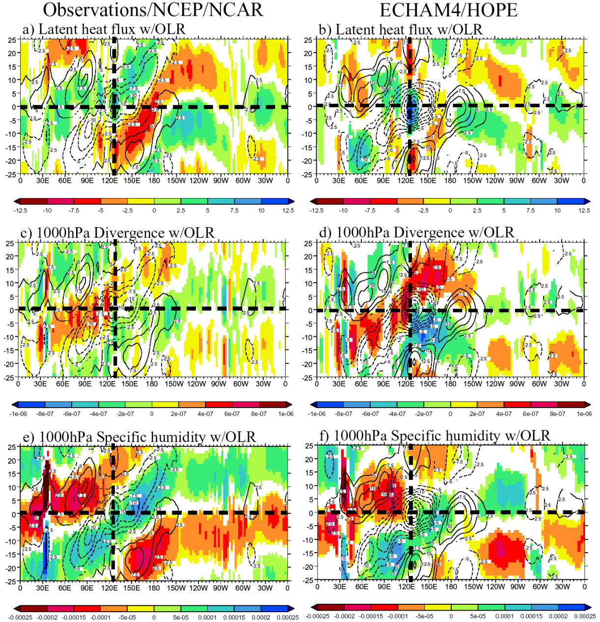
Figure 4 As Fig 3 but for (a-b) latent heat flux ( Wm^{-2} ), (c-d) 1000hPa divergence ( s^{-1} ), and (e-f) 1000hPa specific humidity ( kg\ kg^{-1} )
