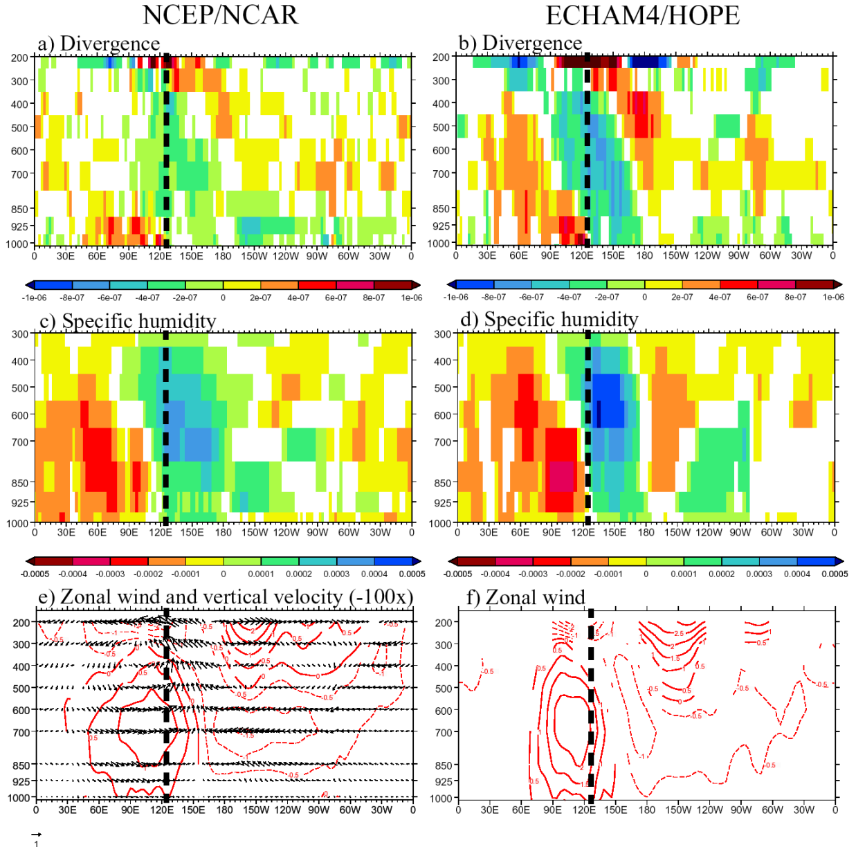
Figure 5 Longitude-height cross-sections of zero time lag linear regressions of PC-1 with 5^{\circ}\text{N} - 5^{\circ}\text{S} averaged 20-100 day bandpass filtered (a) divergence ( \text{s}^{-1} ), (c) specific humidity ( \text{kg kg}^{-1} ), and (e) zonal wind/vertical velocity vectors [note: the vertical velocity ( \text{Pa s}^{-1} ) has been multiplied by -100 to give scaling compatible with the u-winds ( \text{ms}^{-1} )] and contours of the u-wind in increments of 0.5\text{ms}^{-1} . (b), (d), and (f) as (a), (c), and (e) but for ECHAM4/HOPE. Note: in (f) the vertical velocity was unavailable so the vectors are omitted. The vertical dashed line at 125^{\circ}\text{E} is the longitude of the strongest convection in Fig. 2a. Wind vectors are plotted at every other grid point for clarity. Data are plotted for a one standard deviation perturbation of PC-1 where the fit is 5% significant or better assuming each pentad is independent.
