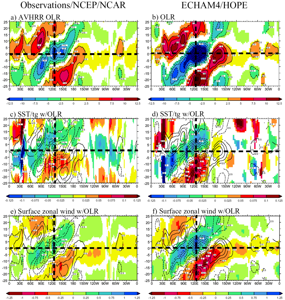
Figure 3 Longitude time-lag plots of the linear regression of PC-1 with 5^{\circ}N-5^{\circ}S averaged 20-100 day bandpass filtered (a) AVHRR OLR ( Wm^{-2} ), (c) SST and ground temperature (K), and (e) 10m zonal wind ( ms^{-1} ). Contours of the OLR regression are plotted on each panel in increments of 2.5Wm^{-2} . (b), (d), and (f) as (a), (c) and (e) but for ECHAM4/HOPE. Time lags run from -25 to 25 Days. The vertical dashed line gives the longitude of strongest convection in EOF-1 (Fig. 2a), and the horizontal dashed line corresponds to zero time lag. Data are plotted for a one standard deviation perturbation of the respective principal components where the fit is 5% significant or better assuming each pentad is independent.
