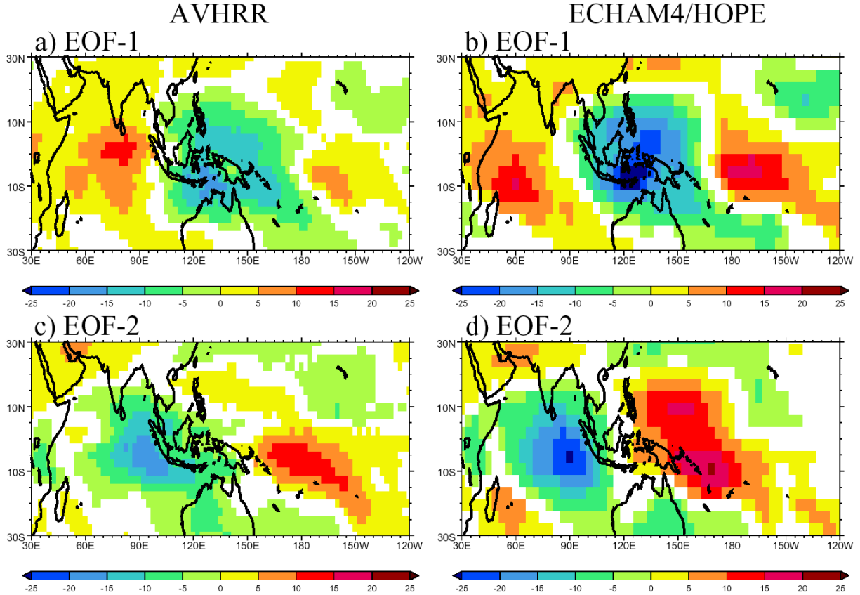
Figure 2 Lag 0 linear regressions of PC-1 with 20-100 day filtered OLR ( \text{Wm}^{-2} ) (a) AVHRR OLR. (b) ECHAM4/HOPE, (c) and (d) as (a) and (b) but for regressions using PC-2. Data are plotted for a one standard deviation perturbation of the respective principal components where the fit is 5% significant or better assuming each pentad is independent.
