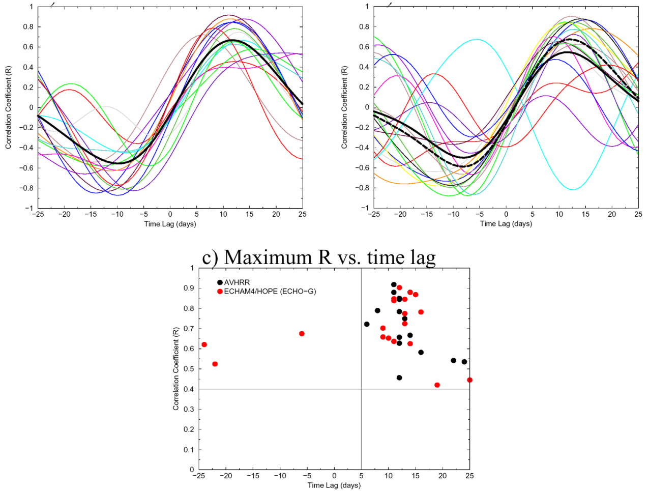
Figure 1 Lead-lag correlation between PC-1 and PC-2 for each winter. Positive correlations at positive time lags indicate that convection over the Indian Ocean leads that over the Western Pacific Ocean. The solid black curve is the average over all years of data. For the model, the dashed black curve is the average for the years that lie in the observed phase-space (upper-right quadrant) of Fig. 1c (a) AVHRR, (b) ECHAM4/HOPE, (c) Phase-space of the maximum positive correlation and its associated time lag for each year of data.
