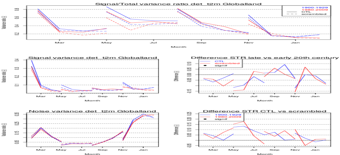
Figure 3: As Figure 2, for detrended temperature
