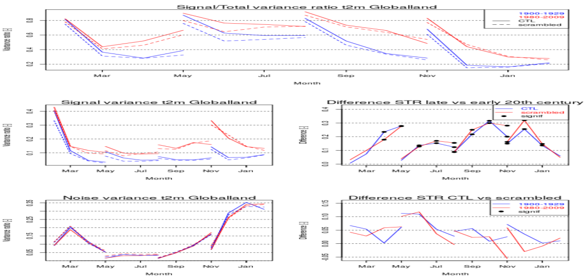
Figure 2: As figure 1 for 2m temperature over land
