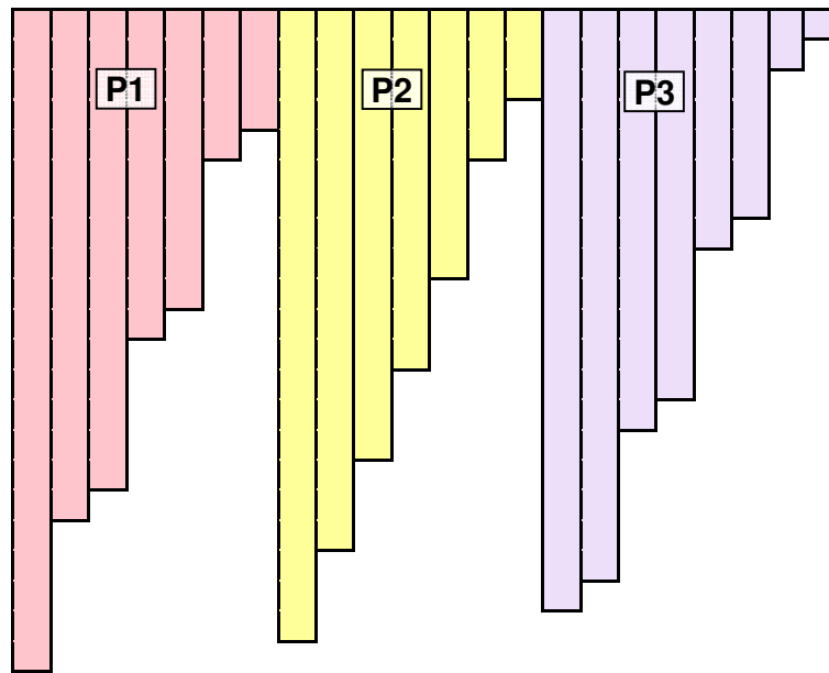
Figure 2.15 Global representation of T21 spectral triangle.
