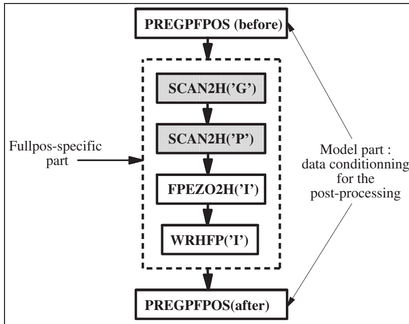
Figure 2.8 Physical fields post-processing: GRIDPFPOS . The greyish areas correspond to model subroutines.
