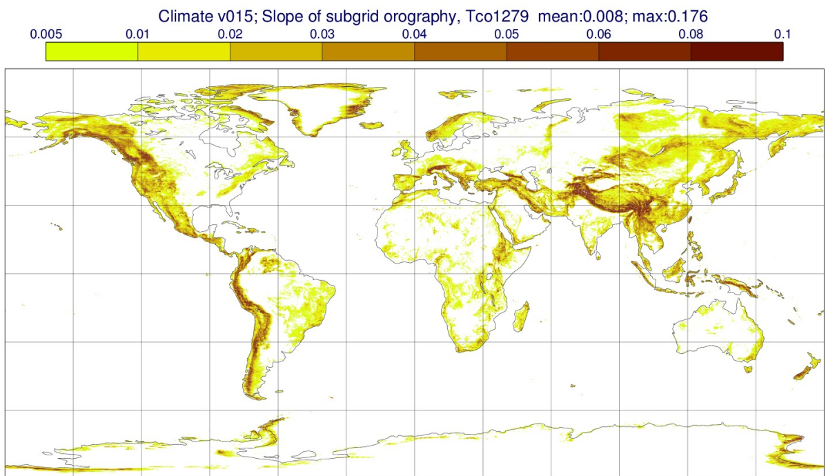
Figure 11.7 Slope \sigma_{\text{GW}} of sub-grid orography.
