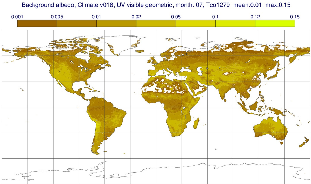
Figure 11.24 Climatological background albedo for July (UV visible, geometric).
