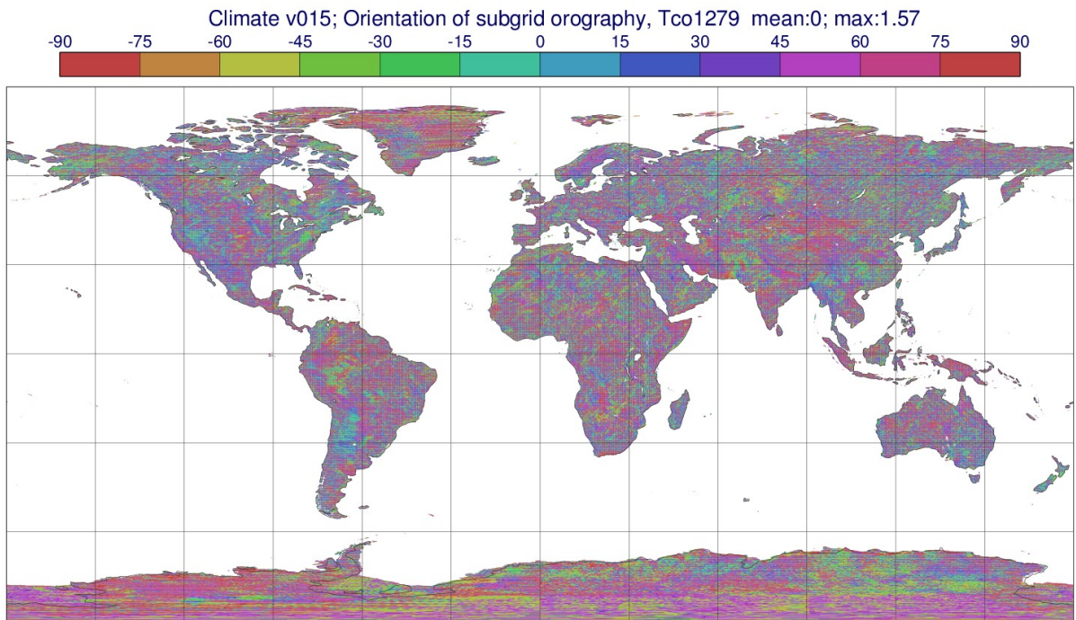
Figure 11.6 Orientation \theta_{\text{GW}} of sub-grid orography. The field is in radians and has values between -\frac{1}{2}\pi and \frac{1}{2}\pi ). For clarity the plot has been converted to degrees with values between -90 and +90 .
