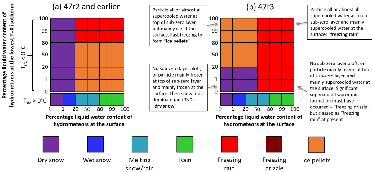
Figure 7.5 Diagnosis of precipitation type from 2m temperature, percentage liquid water content of hydrometeors at the surface and at the lowest T=0^\circ\text{C} isotherm (if present), for (a) Cycles 47r2 and earlier, (b) Cycle 47r3.
