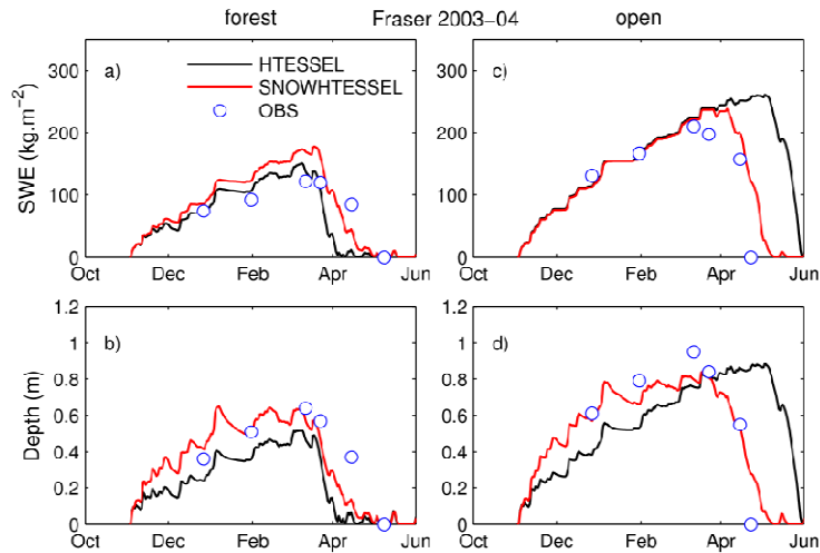
Figure 3 Model-simulated snow mass (a,c) and snow depth(b,d) in SNOWHTESSEL (red) and HTESSEL (black) compared to observations (blue) on SNOWMIP2 Fraser forest (a,b) and open (c,d) site (Colorado)during the 2003-04 winter season.
