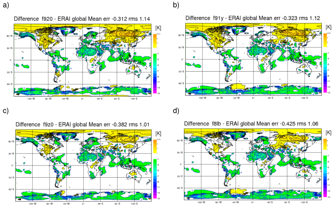
Figure 7: Mean annual 2m temperature errors in long integration compared to ERA-Interim for: (a) TESSSEL (b) HTESSSEL (c) HTESSSELSNOW, (d) SNOWLAIHTESSSEL
