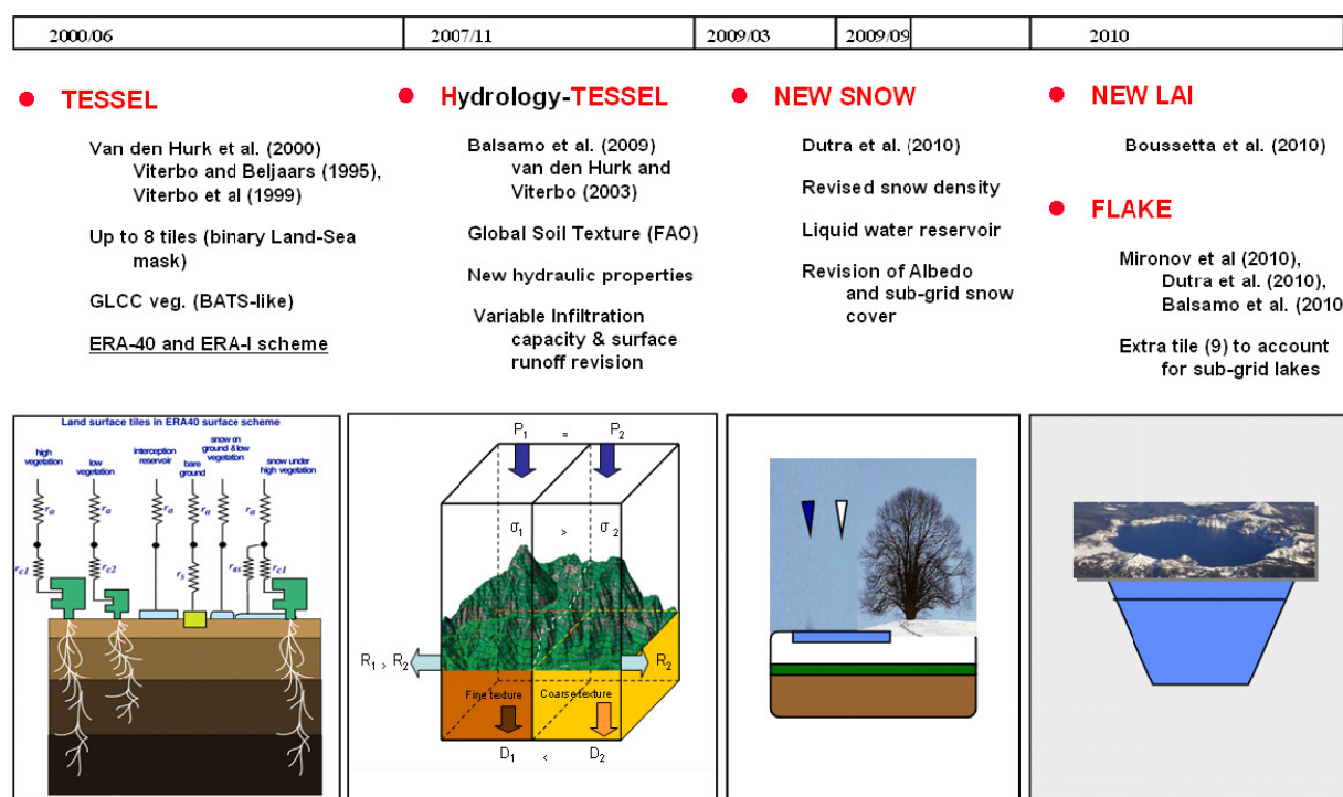
Figure 1: Sketch of the recent revisions to the land surface model with the timeline for activation in the operational IFS.
