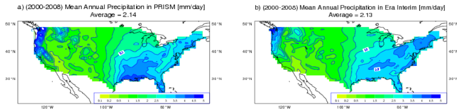
Figure 8: Annual mean precipitation (2000-2008, expressed in mm/day) for a) PRISM, b) ERA-Interim. In panels c) the bias of ERA-Interim and in d) the bias of ERA-Interim-rescaled.
