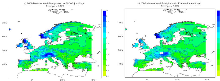
Figure 9: Annual precipitation (in 2000, expressed in mm/day) for a) ELDAS, b) ERA-Interim.
