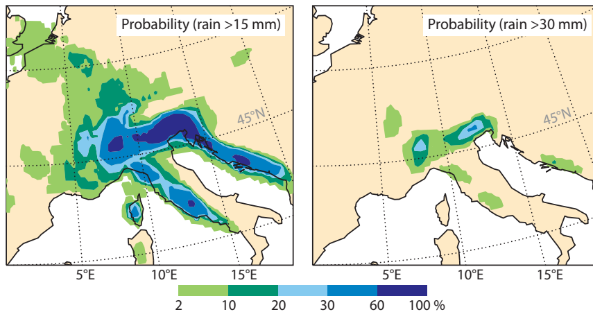
b T+96 to T+144 hour forecasts issued on 23 April
