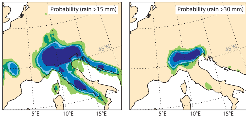
b T+96 to T+144 hour forecasts issued on 23 April
