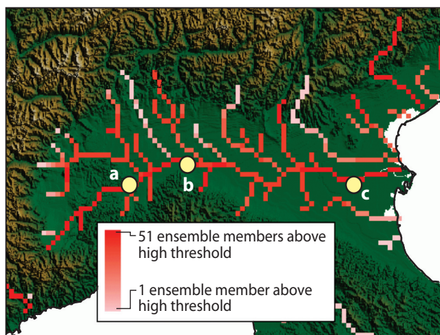
Figure 7 Number of ensemble members based on the ECMWF EPF forecast from 00 UTC on 24 April simulating discharges which exceed the EFAS high alert level for the Po river basin. The circles denote the locations of reporting points as used in Figure 8.
