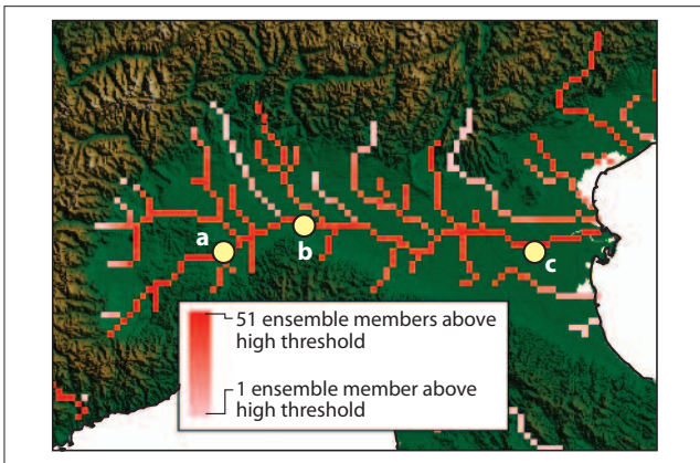
Figure 1 Example of flood probability maps from (a) EFAS showing the combined flood probability of exceeding the EFAS high flood alert from 3–10 days in advance for river pixels only from a forecast from 28 April 2008 and (b) SMHI showing the probability of exceeding the national flood level 1 which corresponds to a 2–10 year return period for May 2008. In both examples the flood threshold levels correspond roughly to return periods of 210 years.
