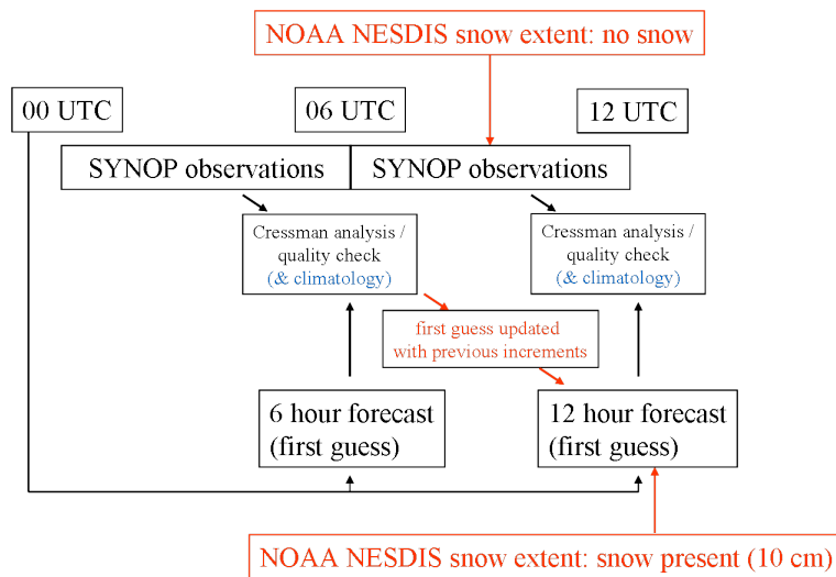
Figure 9: Schematic view of the implementation of the operational snow analysis. The components in blue have been replaced by the components shown in red.
