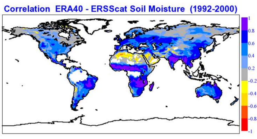
Figure 8: Correlation between ERS scatterometer derived surface soil moisture and ERA-40 top layer soil moisture.
