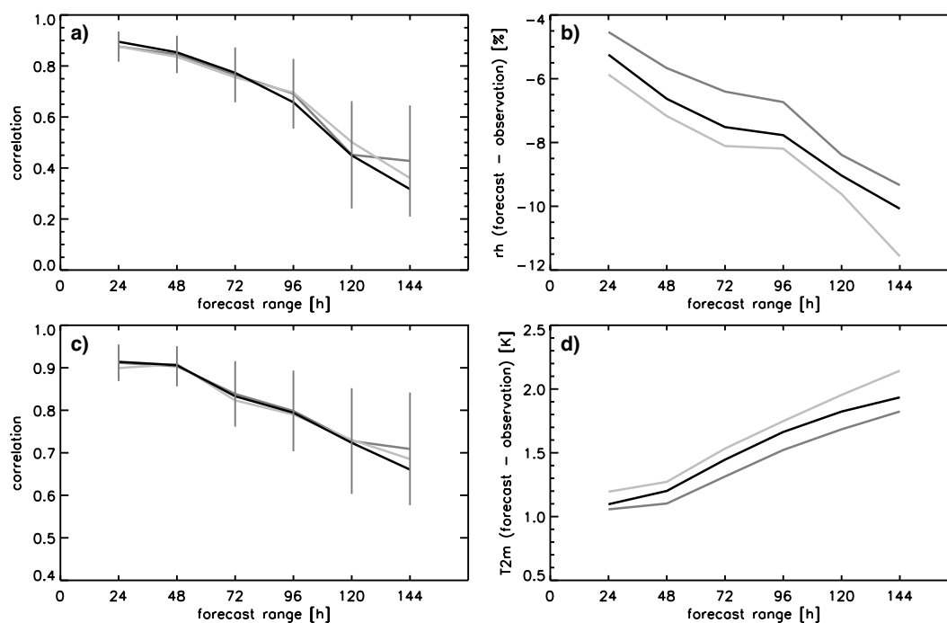
Figure 4: Correlation and bias between forecasts and observations as a function of forecast time. The upper panel presents results for relative humidity, the lower panel air temperature. Forecast basetime is 12 UTC. The CTRL, OL, and NUDGE experiments are represented through dark grey, light grey, and black lines, respectively.
