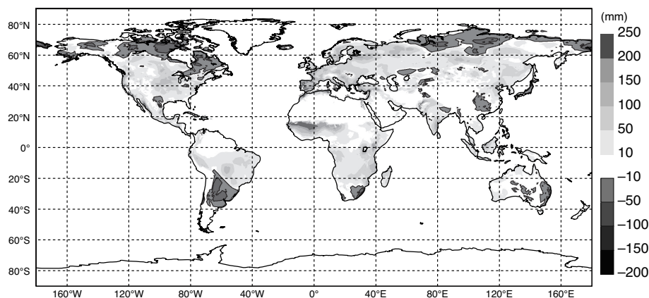
Figure 2: Accumulated root zone (top 1 m soil layer) soil moisture analysis increments (mm) for 2 June to 30 July as computed from the CTRL OI experiment. (from Drusch and Viterbo (2007) )
