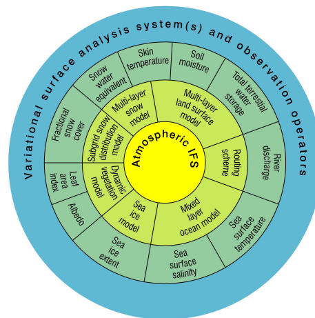
Figure 12: Schematic view on the components of an advanced surface analysis system.
