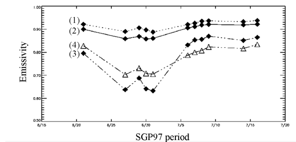
Figure 13: Surface emissivities during SGP97 for the Central Facility Site.
