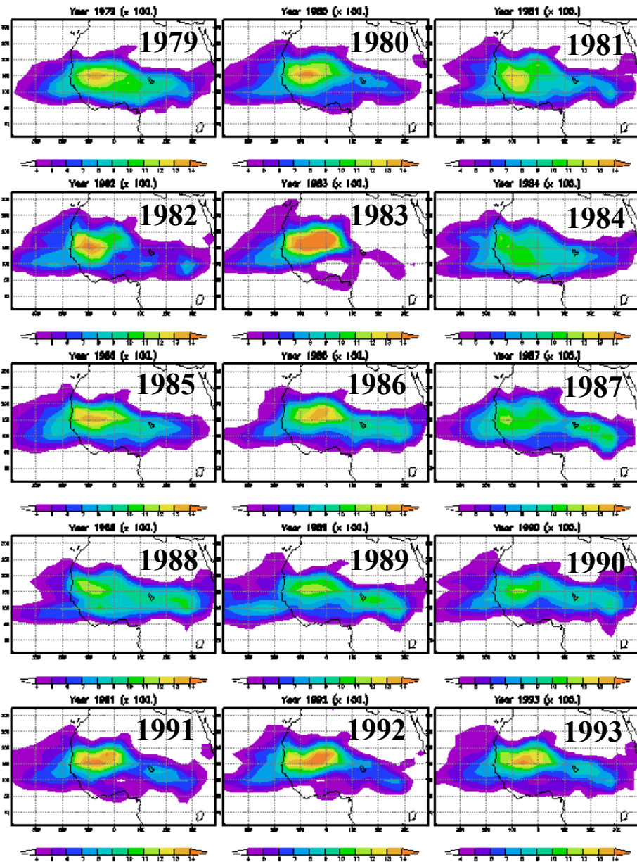
bbx vo85 CEOF: Module of Eigen Vector 1
