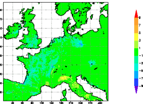
An. Moisture Incr. [kg/m 2 ], L 1, Feb 23, 2003
