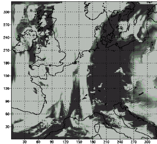
T2m Forecast Error [K], Feb 9, 2003
