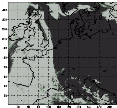
Tot. Cloud Cov. [%], 12 UTC, Feb 23, 2003
