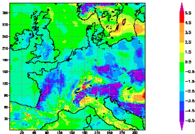
T2m Forecast Error [K], Feb 23, 2003
