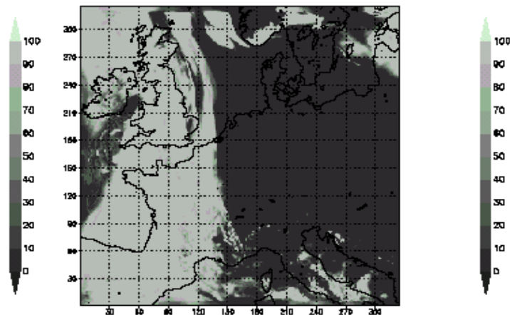
Tot. Cloud Cov. [%], 15 UTC, Feb 23, 2003
