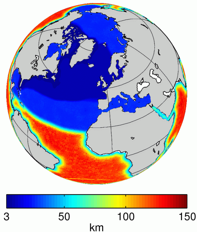
Figure 1: Horizontal resolution (in km) of the FESOM mesh used in the proposed study.
