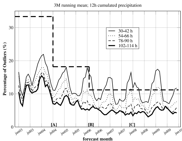
Figure 12: Time-series of the Percentage of Outliers for the 30–42h (solid line), 54–66h (dotted line), 78–90h (dashed-line) and 102–114h (thick-solid line) forecast ranges. A 3-month running mean is applied to improve the readability of the plots. The thick-dashed line indicates the theoretical values of the OUTL. For the meaning of letters [A], [B], [C], refer to the text.
