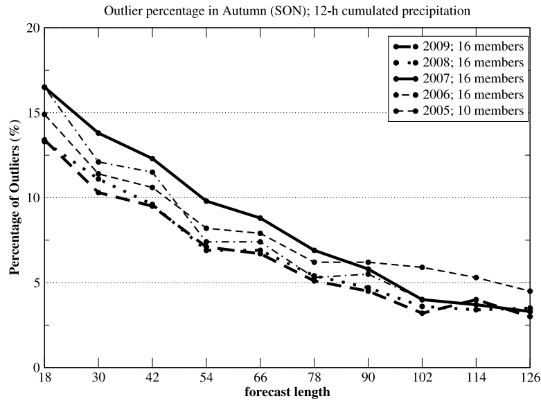
Figure 15: Percentage of Outliers for the forecast ranges of Table ?? and for 5 successive autumns: 2005 (dashed), 2006 (dot-dashed), 2007 (thick-solid), 2008 (thick-dotted) and 2009 (thick-dashed).
