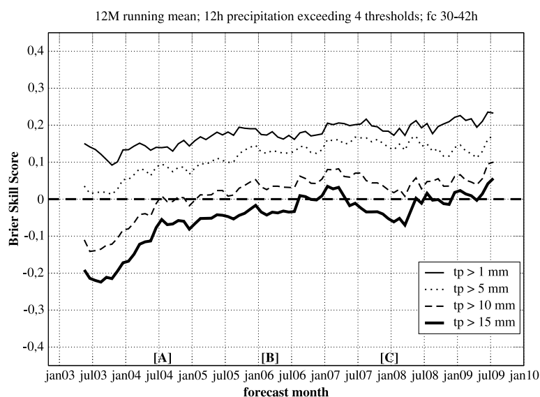
Figure 7: The same as Fig. ??, but with a 12-month running mean applied.
