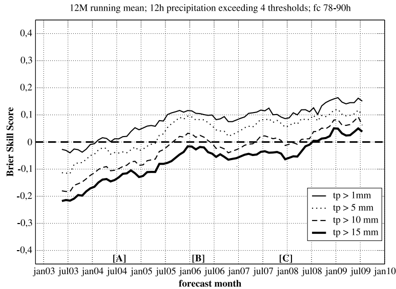
Figure 8: The same as Fig. ??, but for the 78–90 forecast range.
