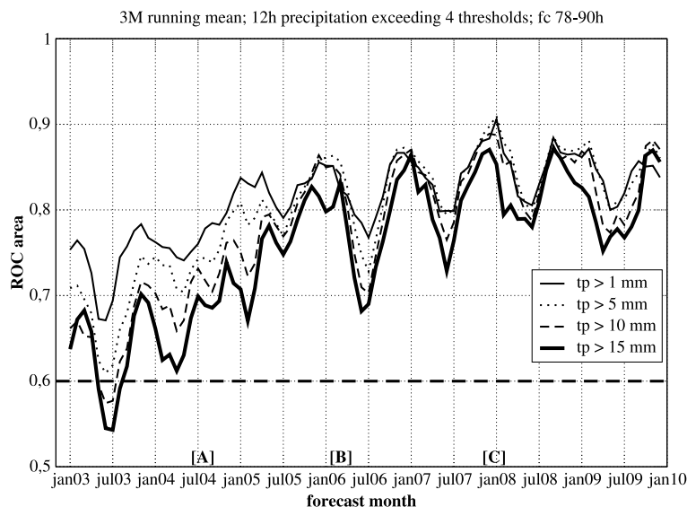
Figure 5: The same as Fig. ??, but for the 78–90h forecast range.
