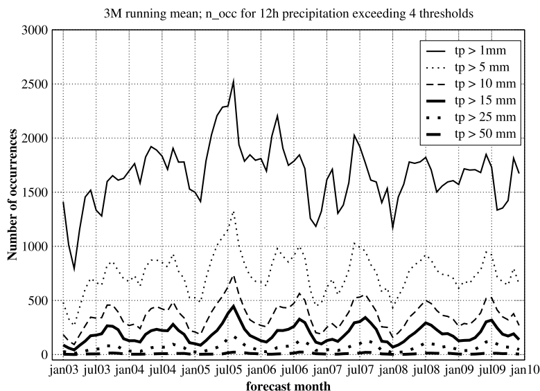
Figure 3: Number of occurrences, according to the reports of the SYNOP stations of Fig. ??, for 12-hour observed precipitation exceeding 4 different thresholds: 1mm/12h (thin–solid line), 5mm/12h (dotted), 10mm/12h (dashed), 15mm/12h (thick–solid), 25mm/12h (thick–dotted) and 50 mm/12h (thick–dashed). A 3-month running mean is applied to improve the readability of the plots.
