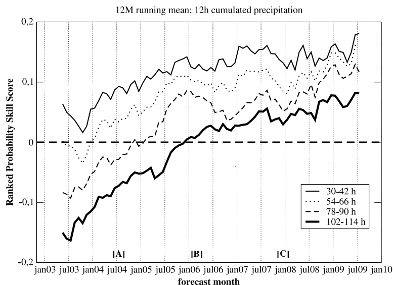
Figure 11: Time-series of the Ranked Probability Skill Score for the 30–42h (solid line), 54–66h (dotted line), 78–90h (dashed-line) and 102–114h (thick-solid line) forecast ranges. A 12-month running mean is applied to improve the readability of the plots. For the meaning of letters [A], [B], [C], refer to the text.
