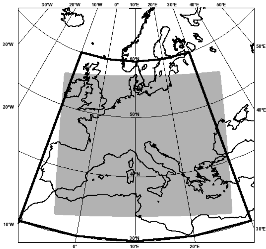
Figure 1: COSMO–LEPS integration domain (gray shaded area) and clustering area (black rectangle).
