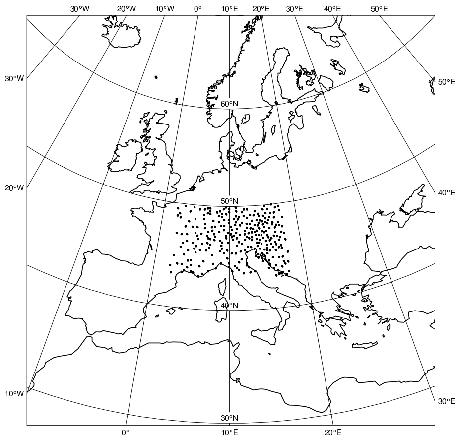
Figure 2: Geographical locations of the SYNOP stations used to verify the performance of COSMO–LEPS. Each station is denoted by a black symbol.
