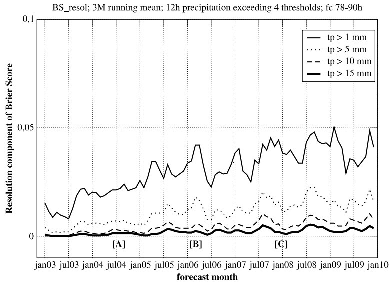
Figure 10: The same as Fig. ??, but for the resolution component of the Brier Score.
