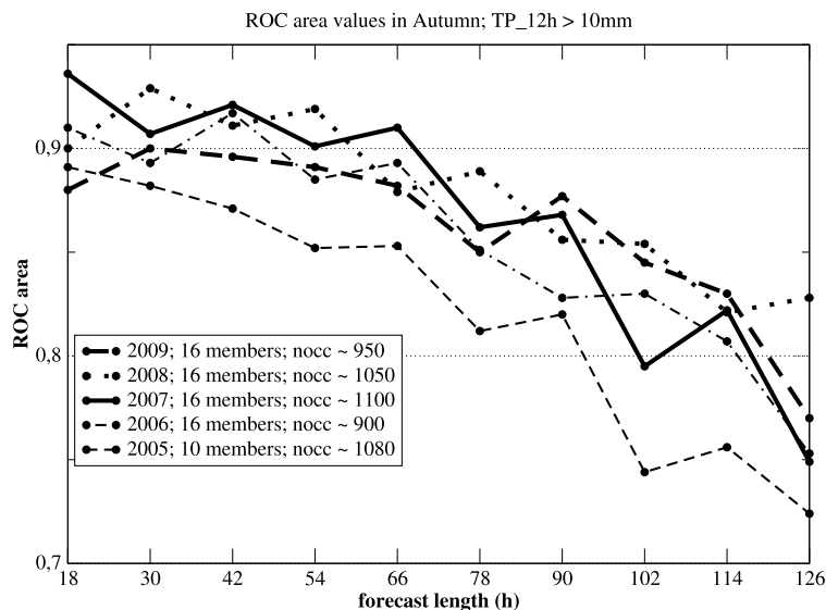
Figure 13: ROC area values for precipitation exceeding 10mm in 12 hours for the forecast ranges of Table ?? and for 5 successive autumns: 2005 (dashed), 2006 (dot-dashed), 2007 (thick-solid), 2008 (thick-dotted) and 2009 (thick-dashed).
